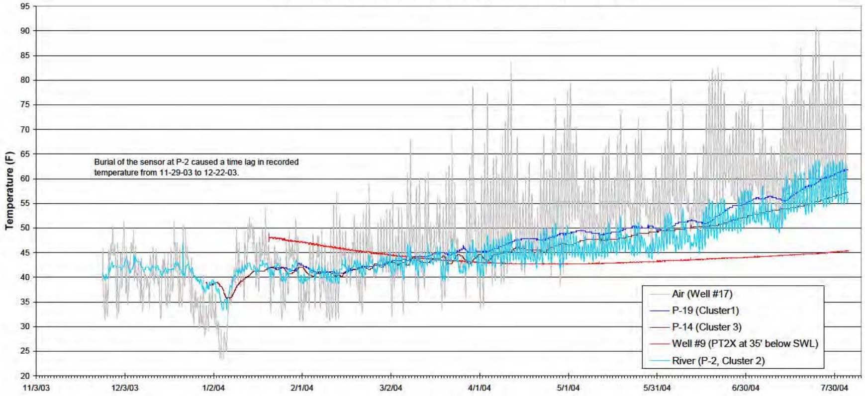
Temperature Data for Clusters 1, 2, and 3 (Reach 1)
