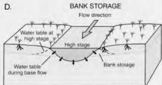
If stream level rises higher than adjacent ground-water levels, stream water moves into the streambanks as bank storage.
