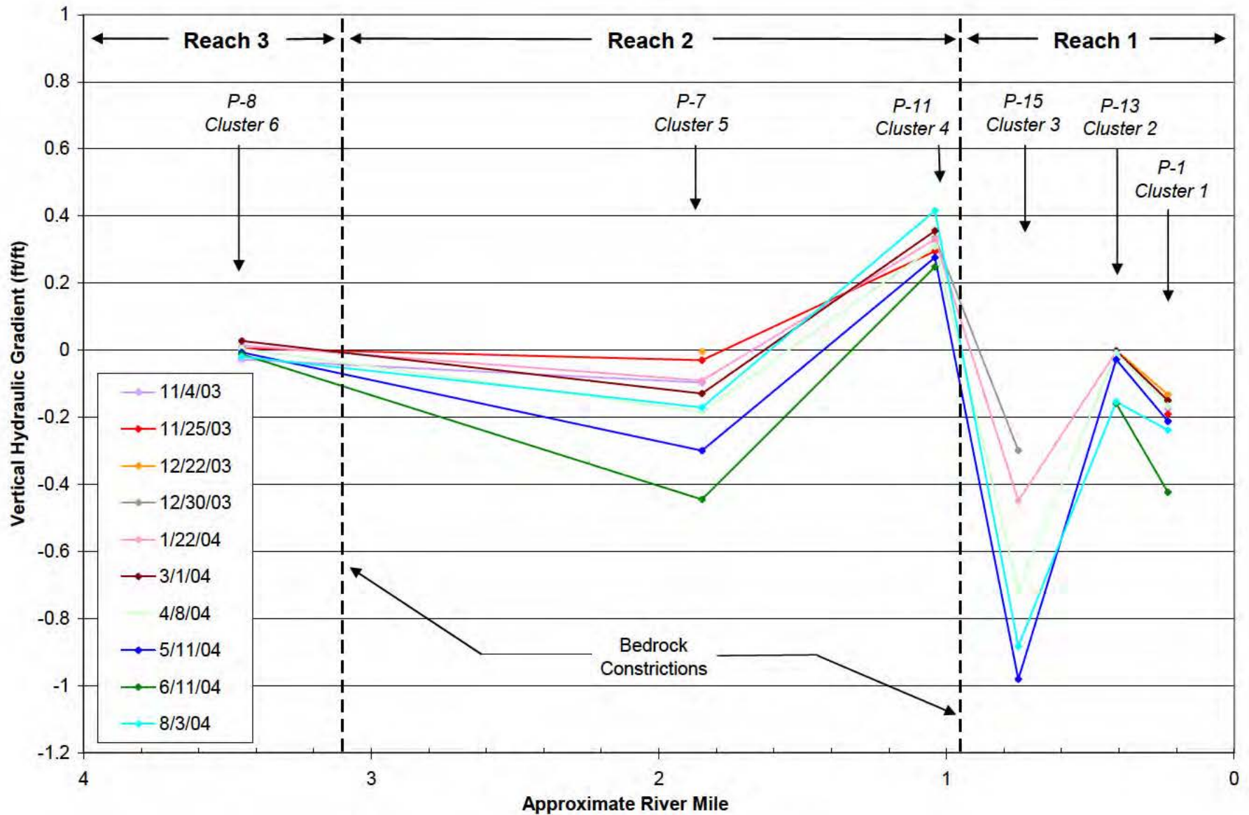
Vertical Hydraulic Gradients Between Surface Water and Groundwater Hydrogeologic Study of the Lower Dosewallips/Brinnon Area Jefferson County, WA
