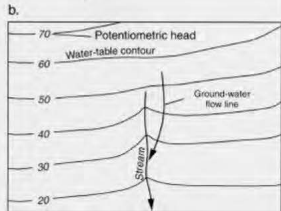
Gaining streams receive water from the ground-water system (B). This can be determined from water-table contour maps because the contour lines point in the upstream direction where they cross the stream (b).
