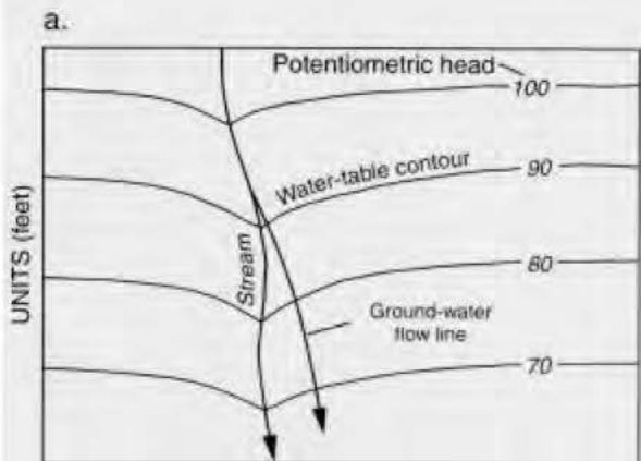
Losing streams lose water to the ground-water system (A). This can be determined from water-table contour maps because the contour lines point in the downstream direction where they cross the stream (a).
