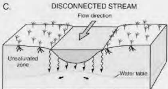
Disconnected streams are separated from the ground-water system by an unsaturated zone.
